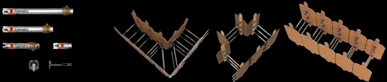
OmniShore Trench Shoring
